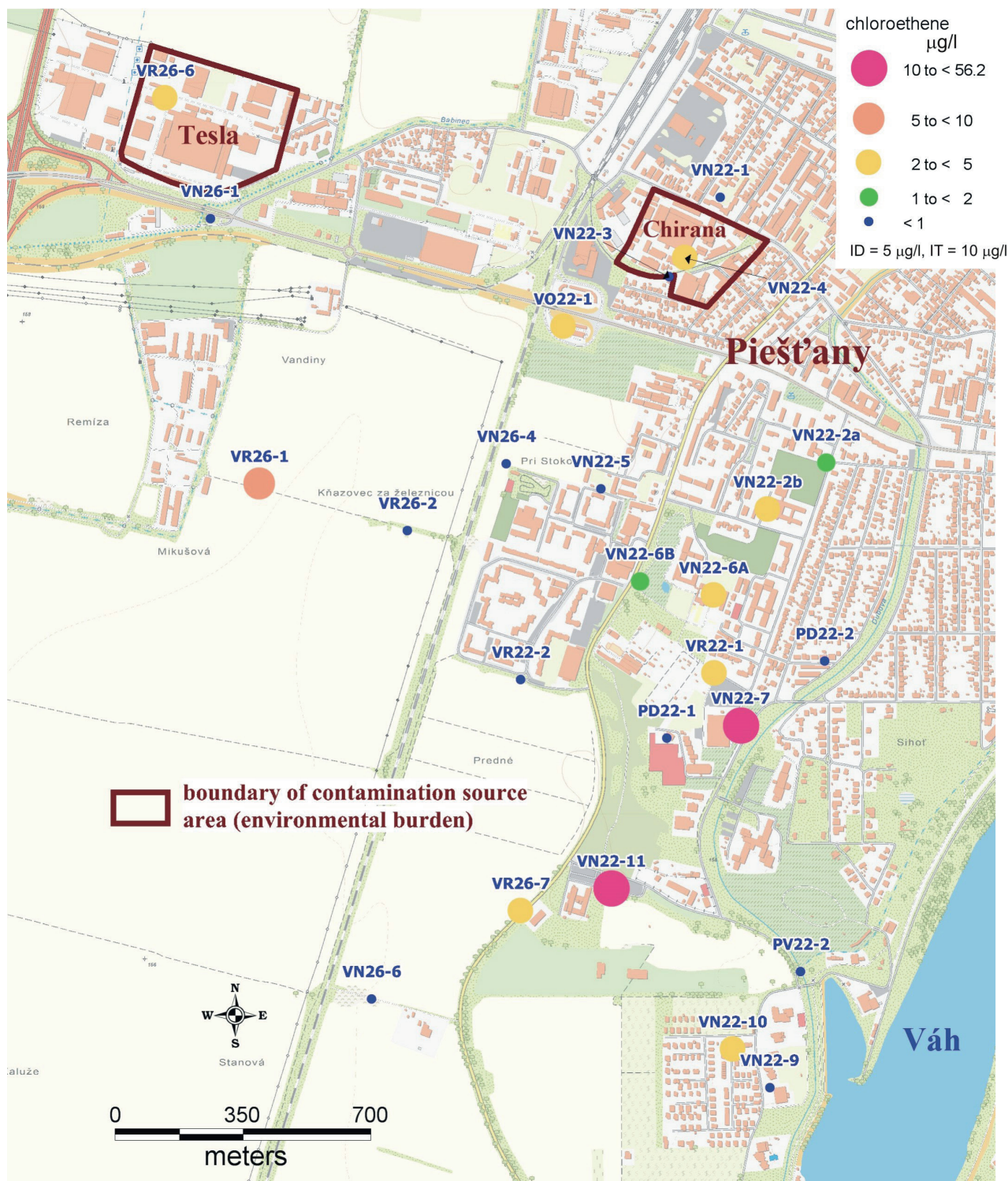
Fig. 1.7 Distribution of chloroethene in groundwaters (median concentrations) – sites Piešťany – former factories Chirana and Tesla (Topographic background: ZBGIS®, The Geodesy, Cartography and Cadastre Authority of the Slovak Republic)
