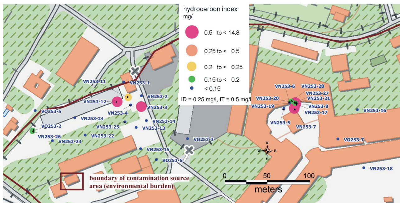
Fig. 1.35 Distribution of hydrocarbon index in groundwaters (median concentrations) – site Komárno – area after the Soviet Army (Topographic background: ZBGIS®, The Geodesy, Cartography and Cadastre Authority of the Slovak Republic)
