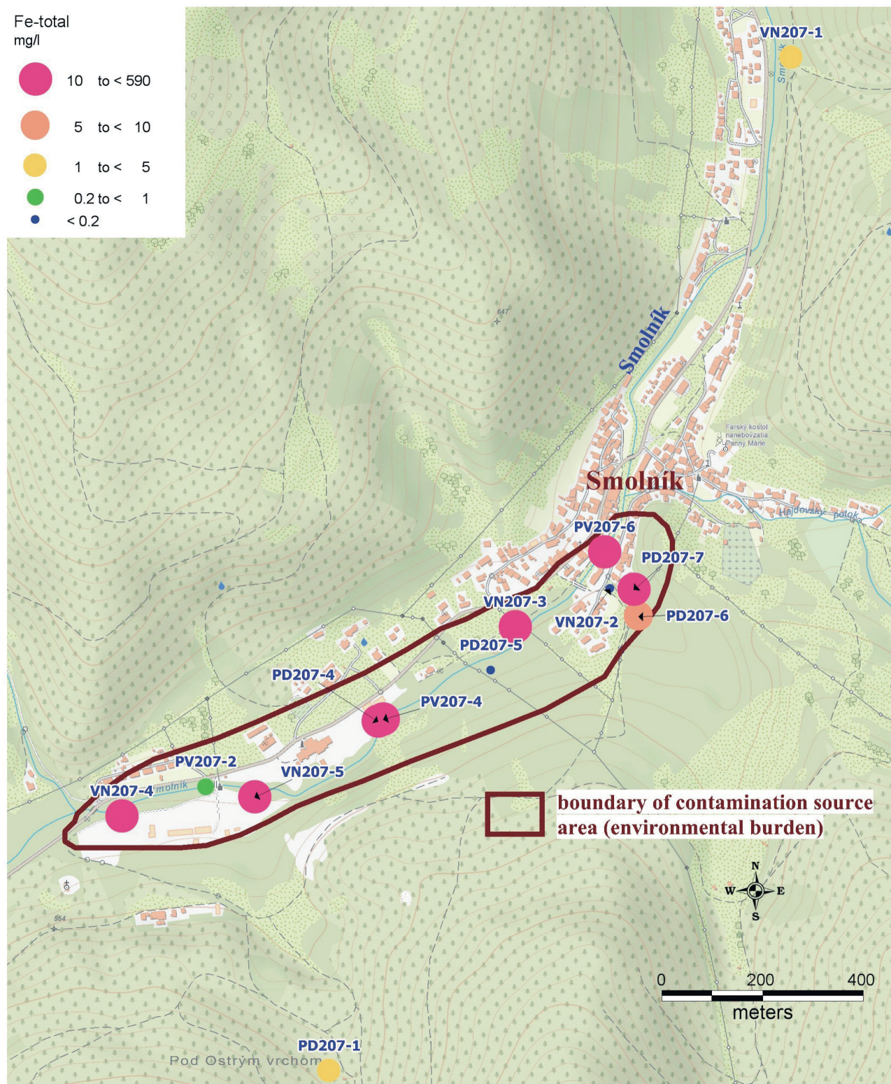
Fig. 1.27 Distribution of Fe in groundwaters (sampled on 27.9.2018) – site Smolník – pyrite ores (Topographic background: ZBGIS®, The Geodesy, Cartography and Cadastre Authority of the Slovak Republic)
