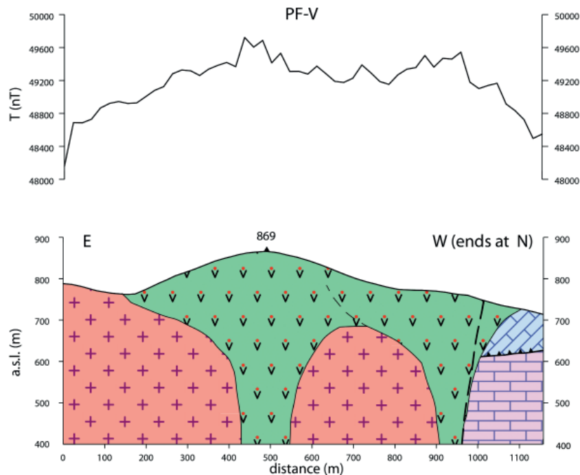
Fig. 27. Geomagnetic profile through the Pálenica body of hypersthene amphibole andesite with garnet: profile PF-V.
