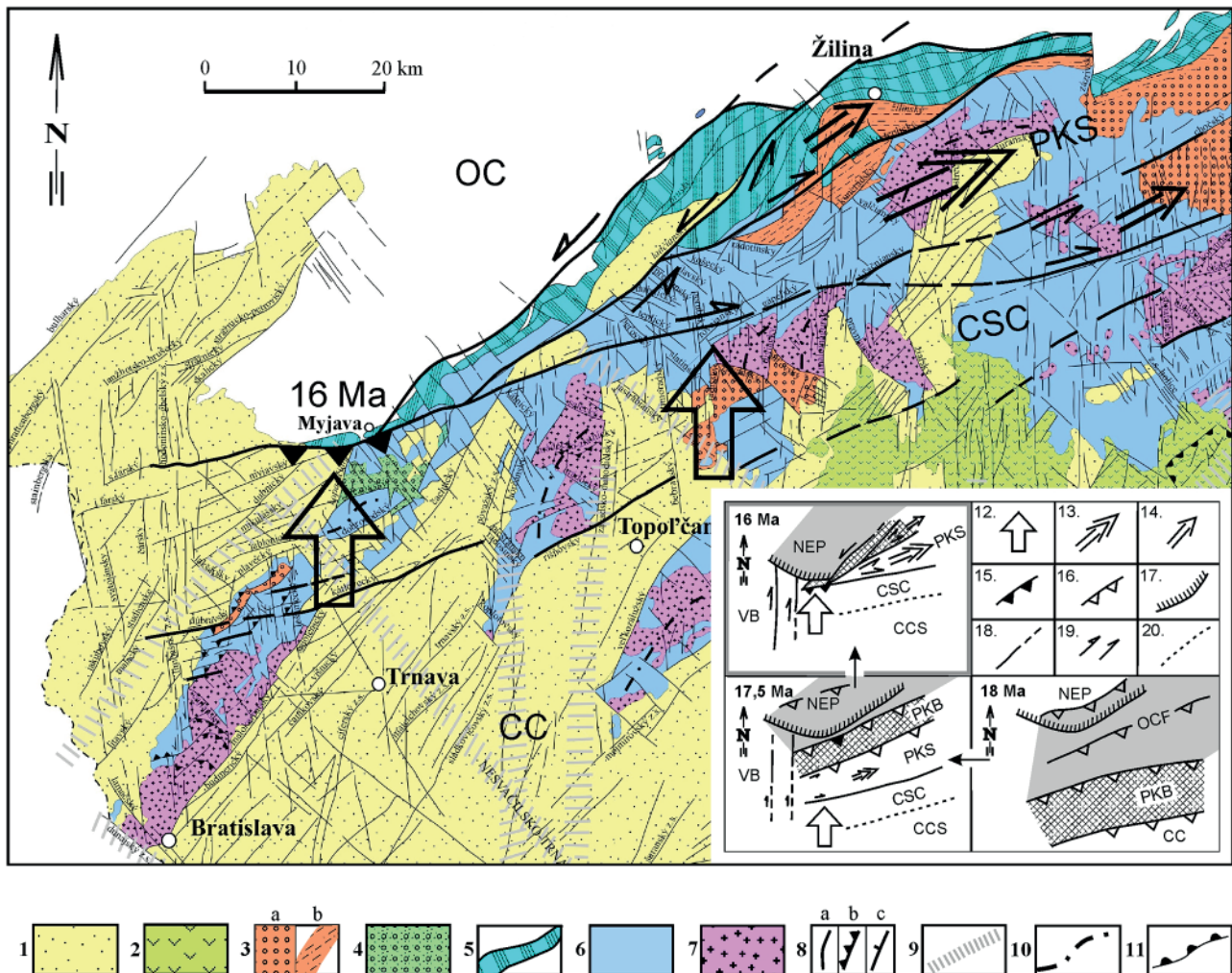
Fig. 3. Interpretation of extrusion tectonics due to a collision of prograding Western Carpathians with a margin of foreland in the depth at the Myjava area (16 Ma ago, after Jiříček, 1979). CC – Central Western Carpathians; CCS – Central Carpathians Segment; CSC – Carpathian Shear Corridor; NEP – North European Plate; OC – Outer Western Carpathians; OCF – Outer Carpathians Flysch units; PKB – Pieniny Klippen Belt; PKS – Peri-Klippen Segment. For explanations 1 – 11 see the legend in Fig. 2; 12 – orogen propagation; 13 – major extrusion; 14 – subsidiary extrusions; 15 – collision with NEP margin; 16 – thrusts; 17 – NEP margin; 18 – activated fault; 19 – fault kinematics; 20 – inactive fault.
