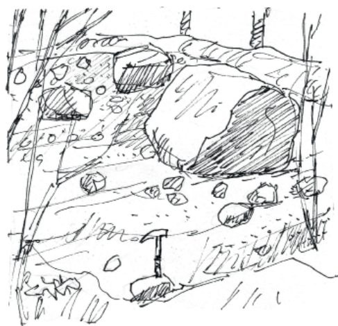
Fig. 55. Coarse to blocky epiclastic volcanic conglomerate is exposed in outcrop with length 15 m and height about 3–4 m on the southern slope of Suchá ridge at level 763 m a.s.l. in the western part of the Hájna hora Hill volcanosedimentary complex. Two fractions of rounded clastic andesite dominate: fraction of well rounded blocks (5–15 cm) deposited in the bedded epiclastic volcanic sandstones and second fraction with blocks with dimensions from 0.7 m up to 1.5 m.
