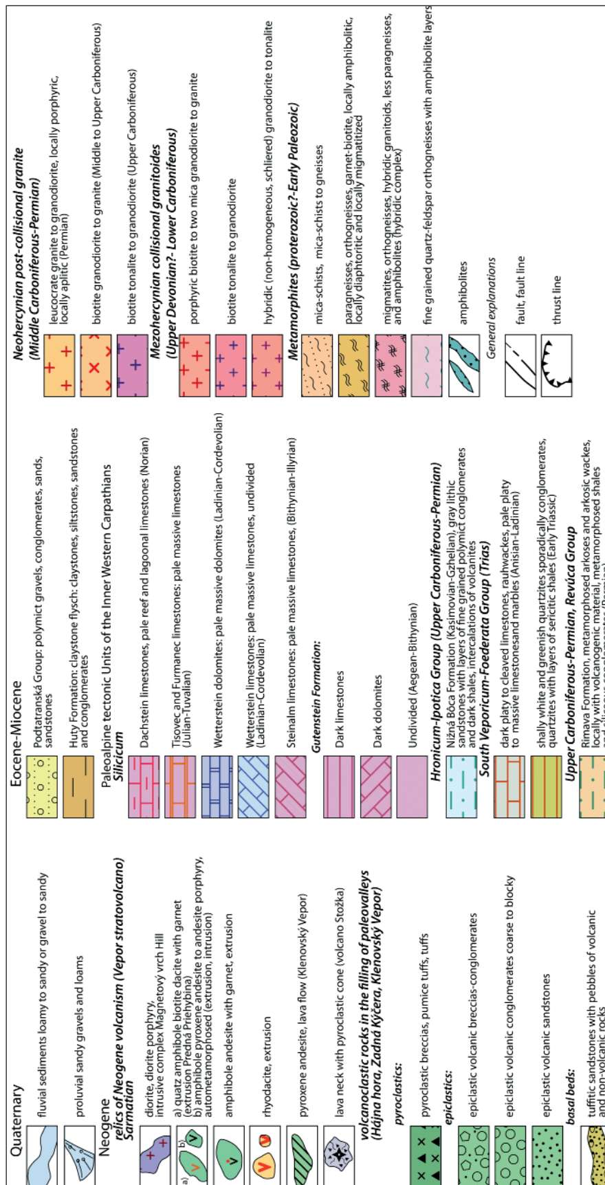
Fig. 6. Scheme of geological setting of the western Veporic unit with situation of relics of the Neogene volcanism.
