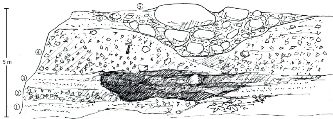
Fig. 69. Volcanoclastic rocks are exposed in rock cliff with length about 15 m and height 5 m on the Zrazy ridge at level 935 m a.s.l. Two layers of fine to medium epiclastic volcanic breccia were distinguished. Lower epiclastic volcanic breccia with angular to subangular fragments up to 5 cm (2) with thickness about 30–50 cm alternates with two layers of coarse-grained epiclastic volcanic sandstones (1, 3). The second thicker body of epiclastic volcanic breccia (4) contains angular to subangular fragments dominantly with dimensions from several cm to 10 cm. Matrix is sandy and tuffaceous. Clastic material is sorted and deposited with normal graded bedding. Body of epiclastic volcanic breccia is dissected in the upper part by erosive channel filled-up with coarse to blocky epiclastic volcanic conglomerate (5).
