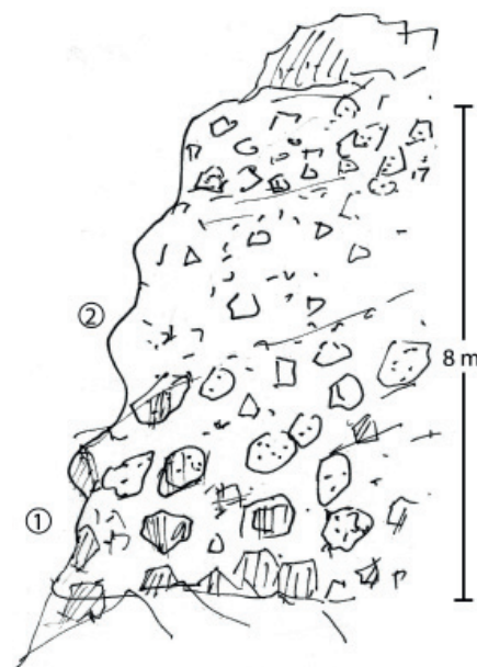
Fig. 61. Reworked pyroclastic breccia on the northern slope of Hájna hora Hill is exposed in several outcrops between altitudes 860–870 m a.s.l. In the lower part of the rock wall there occurs a coarse pyroclastic breccia with vesiculated fragments and spheroidal blocks with diameters from several cm to 30–40 cm (1). Angular fragments are less frequent. Ash-tuff matrix contains large amount fragments of pumices. Deposition of material shows signs of bedding with inclination to NW. Fine to medium pyroclastic material with signs of reverse graded bedding and inclination 15° to NW dominates in the higher part of the outcrop (2).
