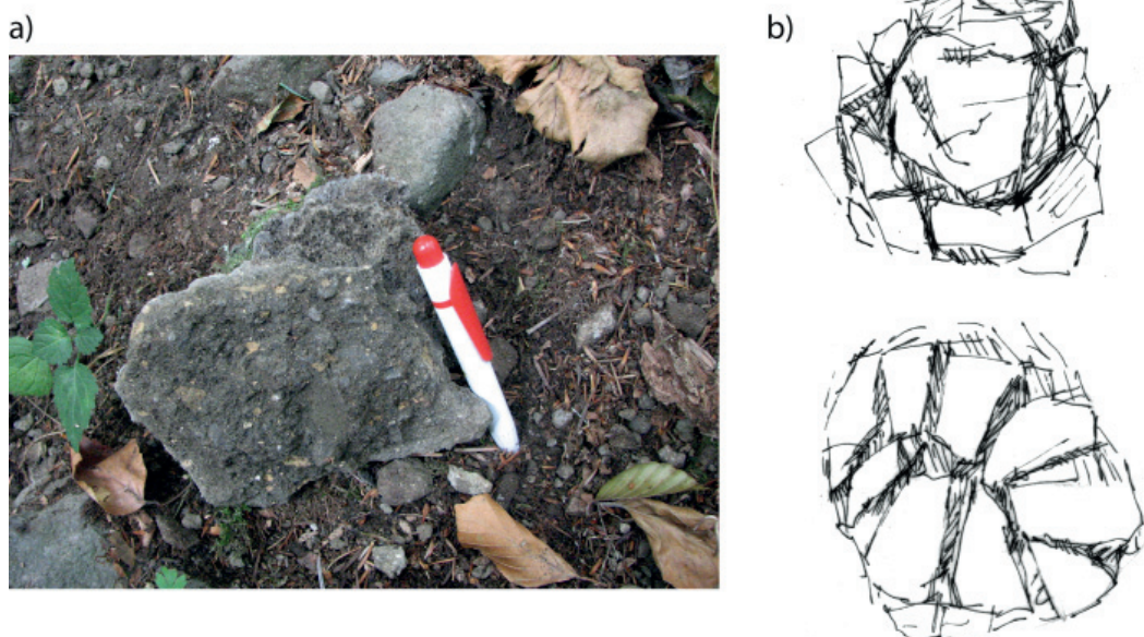
Fig. 59. Matrix of chaotic breccia contains small fragments of pumice and larger fragments of vesiculated andesite. The outer boundary of vesiculated fragments is obscured due to welding with matrix (a). Radial and partly concentric jointing of blocks is result of disintegration during movement in the pyroclastic flow (b).
