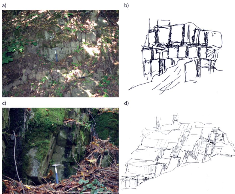
Fig. 8. Regular blocky jointing of inhomogeneous diorite porphyry (DiPN) at the northern edge of the A 1 segment (a, b). Block jointing of medium-grained diorite (Di1) in the northern part of the segment A 1 (c, d).
