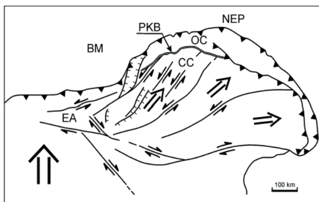
Fig. 1. A concept of Miocene lateral extrusion kinematics with prominent strike-slip and extensional faults (according to Ratschbacher et al., 1991). BM – Bohemian Massif; CC – Central Western Carpathians (Internal Carpathians); EA – Eastern Alps; NEP – North European Platform; OC – Outer Western Carpathians (External Carpathians); PKB – Pieniny Klippen Belt.
