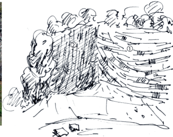
Fig. 26. Inner structure of extrusive complex Pálenica exposed in the quarry on western slope of the Pálenica valley. On the right side of the quarry wall there is andesite with fan-like structure of fluidity planes, photo (a) and scheme (b/1). In the left side of the quarry wall a steep inclination of fluidity plane indicates ascending (intrusion) of younger extrusive body, photo (a) and scheme (b/2).
