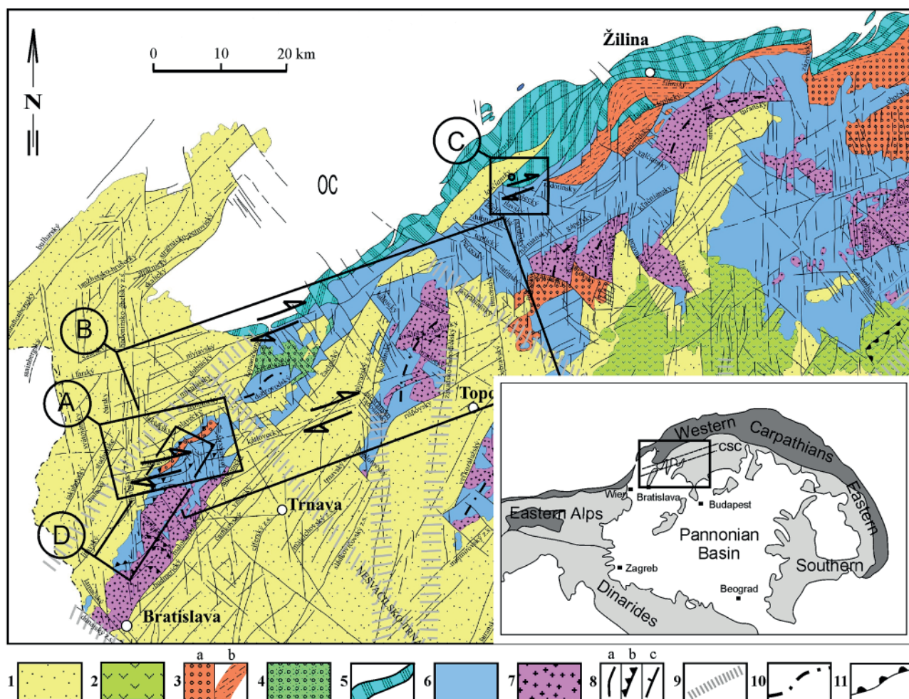
Fig. 2. NW part of Western Carpathians internides with interpreted major post-Cretaceous dislocations (Marko, 2002) and indications of orogen-parallel dextral strike-slips described in literature (A: Marko et al., 1990; B: Fodor, 1995; Fodor et al., 1999; Kováč et al., 1997; Pospíšil, 1990; C: Marko and Hók, 2008; Šimonová and Plašienka, 2011; D: Plašienka, 1990). 1 – Neogene sediments; 2 – Miocene volcanites; 3 – Paleogene sediments in: a – internal position; b – peri-klippen position; 4 – Late Cretaceous sediments (Gosau Group); 5 – Pieniny Klippen Belt units; 6 – undivided Mesozoic units and Late Paleozoic cover; 7 – crystalline basement of core mountains; 8 – faults: a – nonspecified, b – reverse, c – normal; 9 – deep seated discontinuities detected by geophysics; 10 – axes of morpho-structural elevations; 11 – fault margin of volcanic caldera; CSC – Carpathian Shear Corridor; OC – Outer Western Carpathians (flysch belt).
