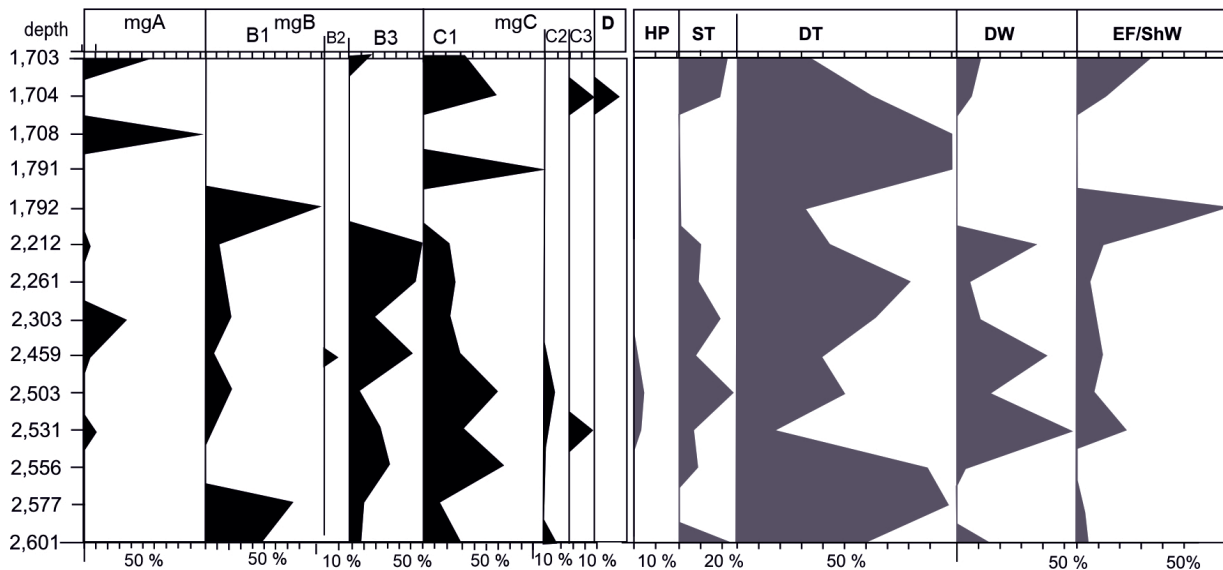
Fig. 7. Relative abundances of palaeoecologically significant groups of benthic foraminifera in samples from the Dubov -2 well. (Left) Morphogroups of agglutinated foraminifera adapted from Murray et al. (2011). (Right) Palaeoecological groups of benthic foraminifera based on Murray (2006) and other authors. Abbreviations: HP – high productivity; DT – dysoxia-tolerant taxa; DW – deep-water taxa; EF/ShW – epifaunal/shallow-water taxa.
