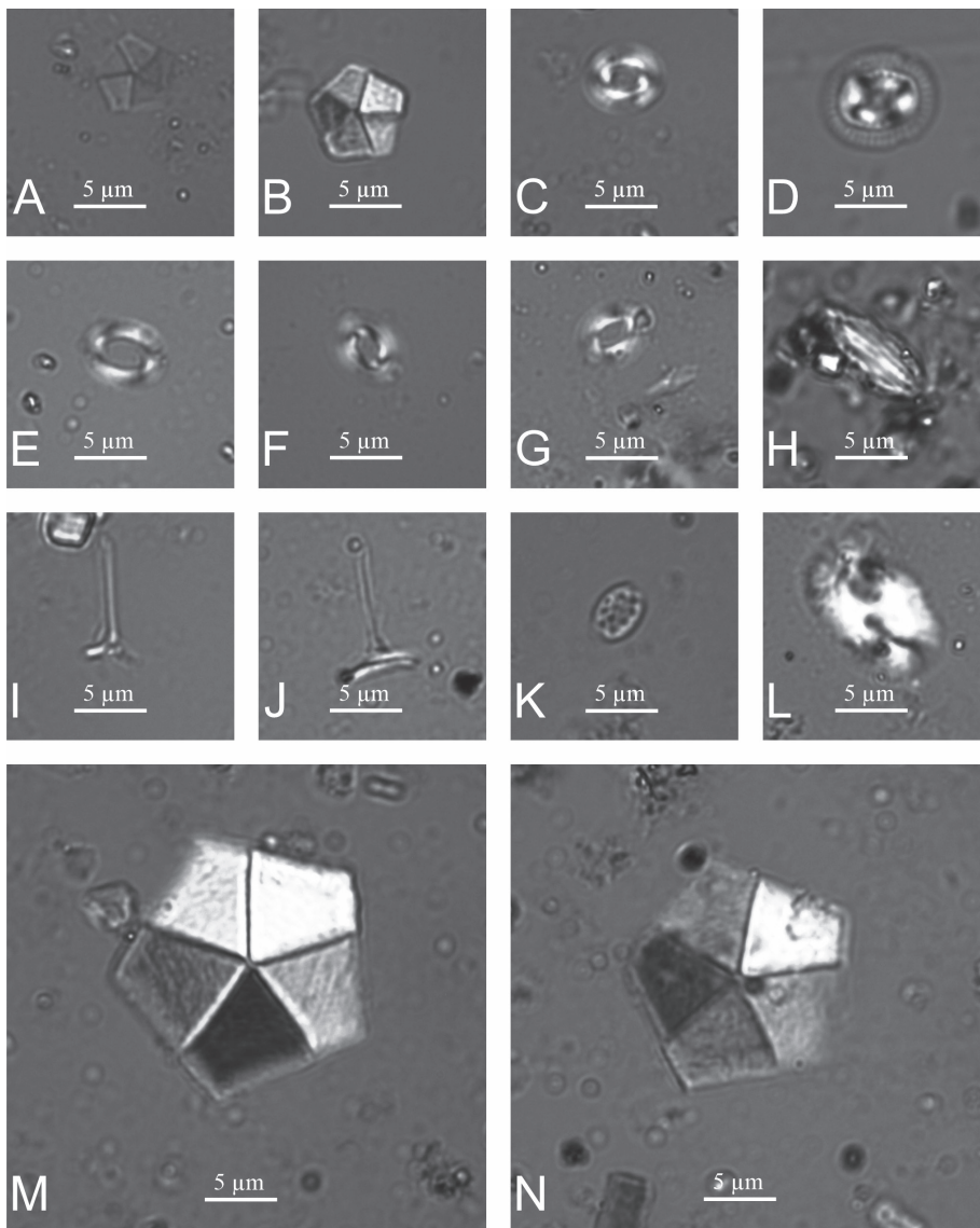
Fig. 6. Stratigraphically important calcareous nannoplankton in the samples studied.
