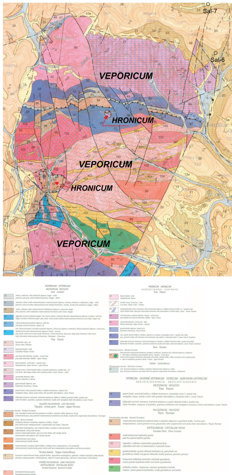
Fig. 6. A section from the geological map of Branisko and Čierna hora (Polák et al., 1996) with explanations and marking of the presumed Veporic structures.
