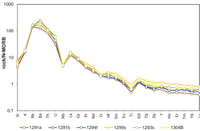
Fig. 7. Multi-element diagram (spiderogram; sensu Sun & McDonough, 1989). Contents of elements are normalized to N-MORB.
