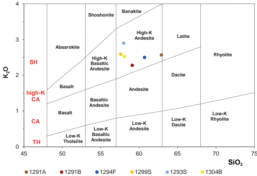
Fig. 6. Position of studied samples in classification diagram of SiO 2 vs. K 2 O (sensu Pecerrillo & Taylor, 1976). Petrogenetic series: TH – tholeiitic, CA – calc-alkaline, high-K CA – high-potassium calc-alkaline, SH – shoshonitic.
