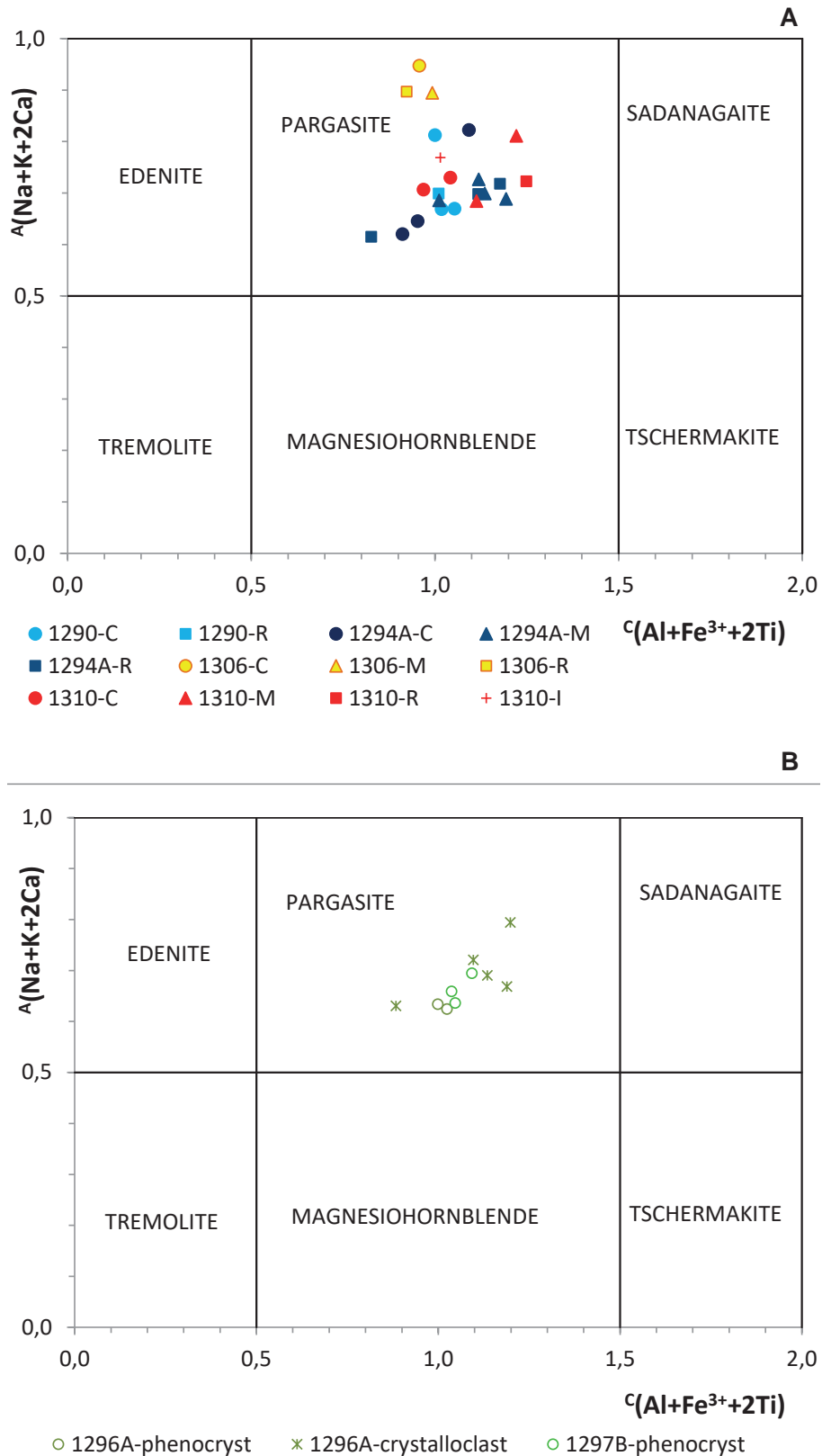
Fig. 13. Classification diagram for amphiboles (Hawthorne et al., 2012) for Fe^{3+} min. Diagram A is for amphiboles in andesites, diagram B for amphiboles in tuff. C – core, M – mantle, R – rim of pyroxene, I – inclusion of amphibole in another mineral.
