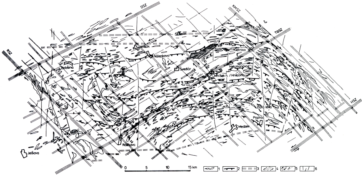
Fig. 4. Schematic visualization of shear zones of Gemericum (Grecula et al., 1990; published with permission), representing the milestone in understanding of the role of Cenozoic Alpine faulting in the territory of the Internal Western Carpathians. RSZ – the Rejdová shear zone, DSZ – the Dobšiná shear zone, KMSZ – the Košice-Margecany shear zone, TGSZ – the Transgemeric shear zone, HSZ – the Hodkovce shear zone; 1 – course of lithological units, 2 – nappes, 3 – Alpine rejuvenated older generation shear zones, 4 – principal Alpine shear zones, 5 – shear zones of lower order, 6 – faults with a pure shear character (the youngest ones).
