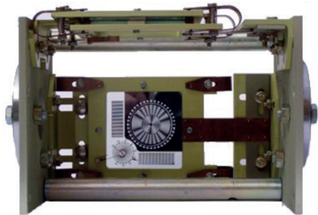
Fig. 2. Mechanical-optical dilatometer of TM-71 type.
