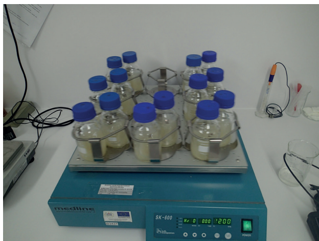
Fig. 10. Kinetic study of As sorption onto zeolite in batch conditions.
