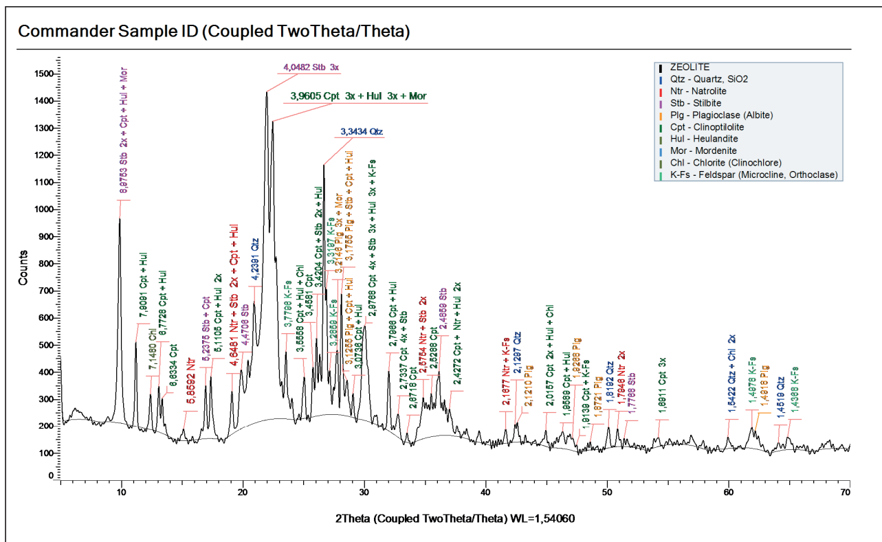
Fig. 8. XRD pattern of zeolite.
