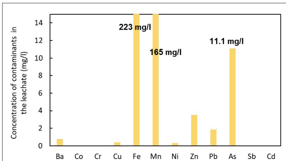
Fig. 7. Concentration of studied contaminants in leachates after the SBET test.
