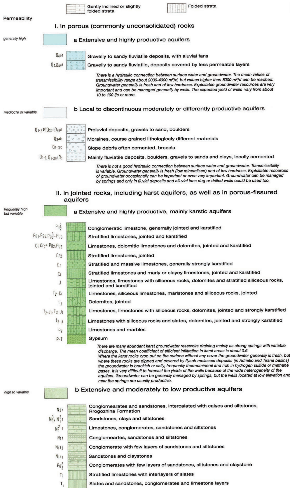
Fig. 4a. Hydrogeological map of Albania sc. 1:200,000; hydrogeological classification of the rocks – first part.
