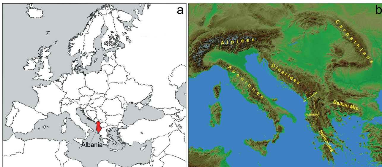
Fig. 1. a) Location map of Albania, b) Tectonic position of Albania.
