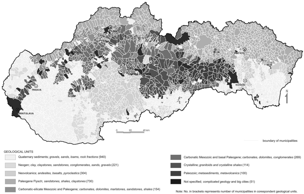
Fig. 1 Division of geological structure of the Slovak Republic in main geological units
