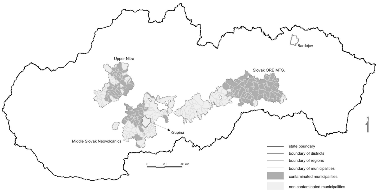
Fig. 2 Contaminated and noncontaminated areas of the Slovak Republic
